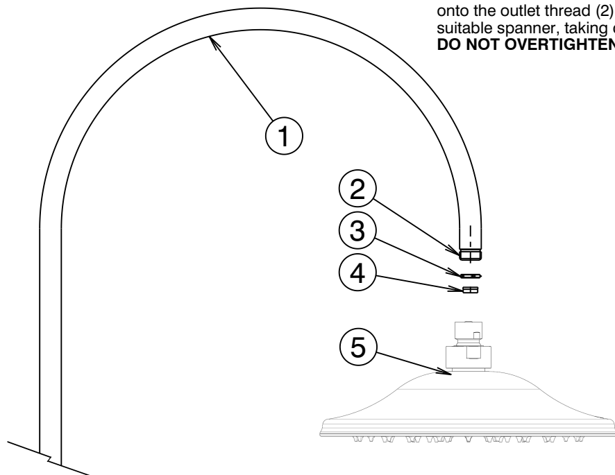
SHOWERHEAD INSTALLATION
