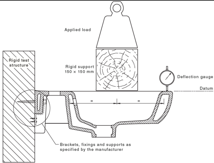
Figure B.1 — Typical arrangement for load safety test for washbasin
